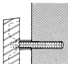
PM-1 Projected mount with collars and threaded studs set in adhesive
