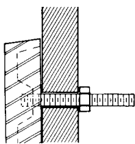
FM-4A Same as FM-4 bolted from the rear (no adhesive)
