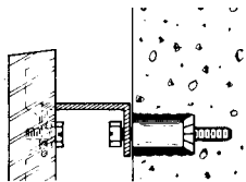
PM-2 Projected Mount with brackets (minimum projection 2")
