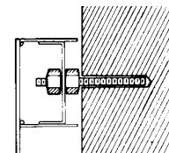
FABRICATED LETTERS Adaptable to any stud-type mounting shown.
